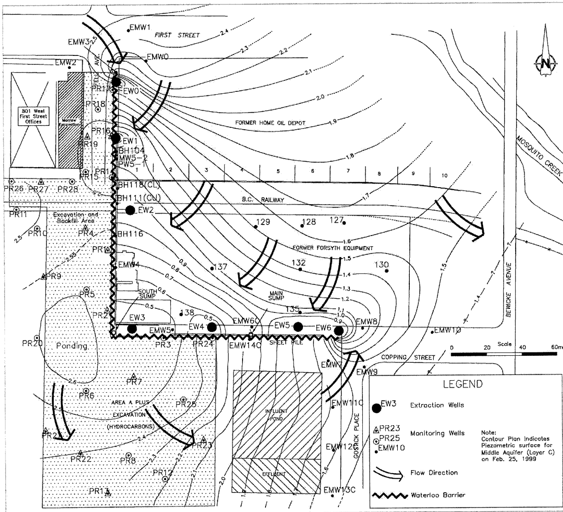
Figure 4. Performance monitoring of hydraulic barrier system (Feb. 25, 1999).
