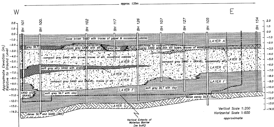
Figure 2. Hydrostratigraphic section along East-West run of Waterloo Barrier.
