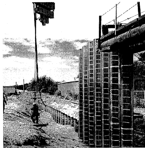
Photo 1. Driving WEZ-95 sheet pile using driving frame.
